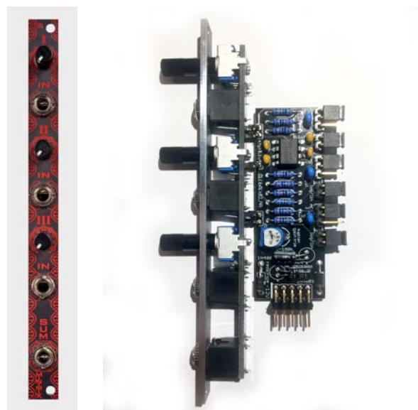
Close-up of the Minimix front & side view
